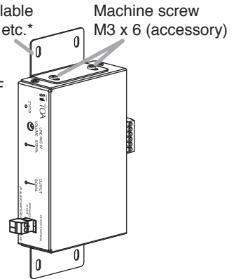
M3 x 6 (accessory) * Plate thickness 1 to 3 mm (0.04" to 0.12")
